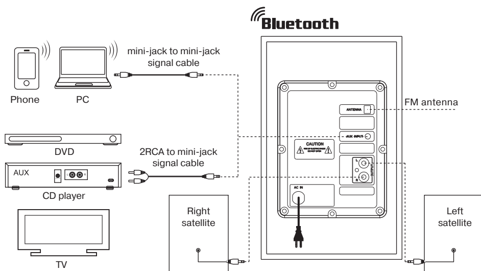
Fig. 4. Connection diagram
